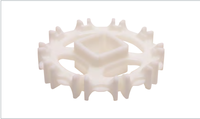
OEM Part Number: 31.2810 Sprocket 6" 10 Tooth Tarheel Part Number: CP-007
