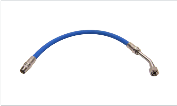
OEM Part Number: 0858.0050.000.51 Hose for Birdwasher Tarheel Part Number: CP-1320
