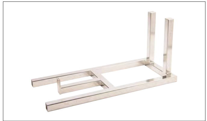
OEM Part Number: 08.32.000.001M Motor Frame Modified Tarheel Part Number: CP-1012M
