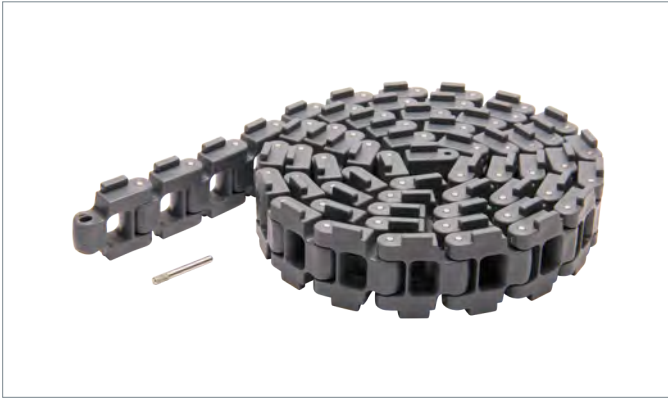
OEM Part Number: A2E5-49DXX1-LS-000 Knuckle Chain with Track Guide (10 foot/piece) - Grey Tarheel Part Number: CP-455
