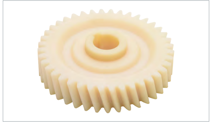
OEM Part Number: 364053003 LH White Gear 40 Tooth Tarheel Part Number: CP-109
